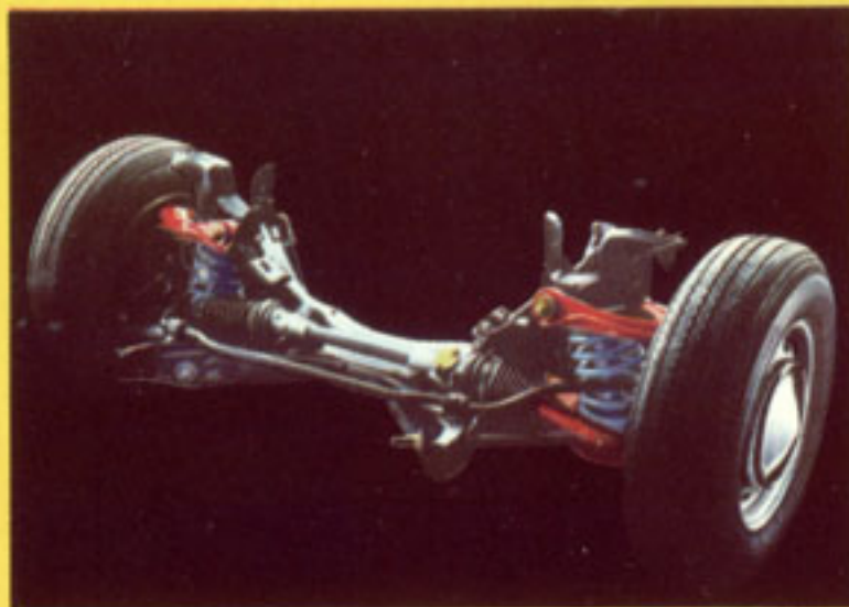
The elaborate suspension system of the Consul Estate: all four wheels independently suspended.
