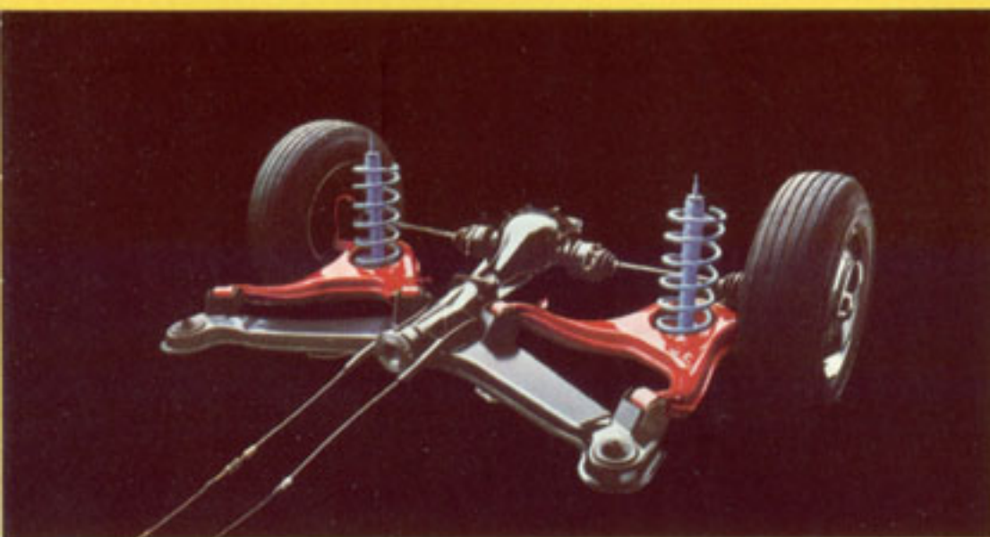
The elaborate suspension system of the Consul Estate: all four wheels independently suspended.
